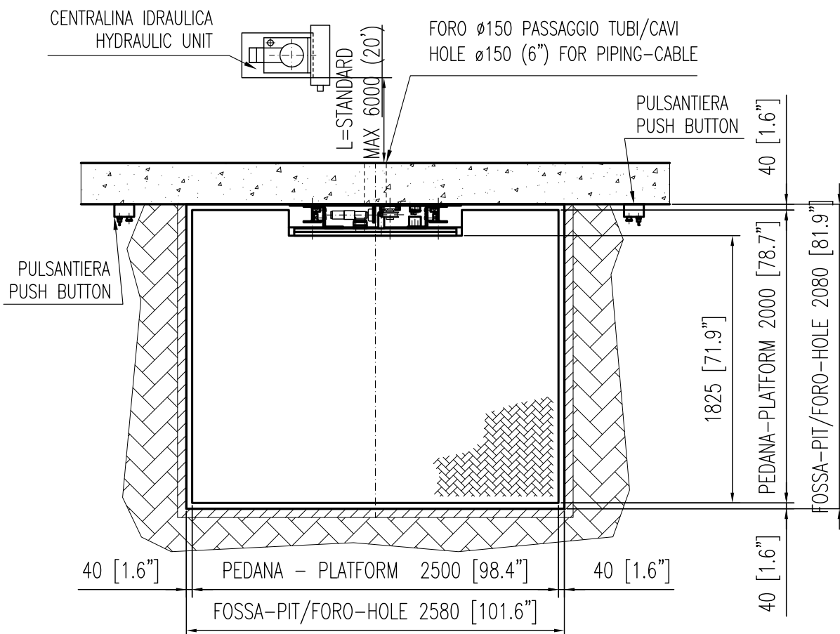
VISTA IN PIANTA PLAN VIEW
