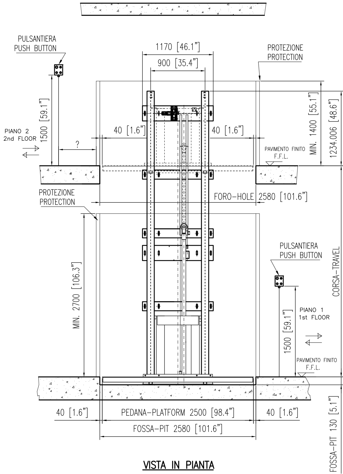
VISTA FRONTALE FRONTAL VIEW
