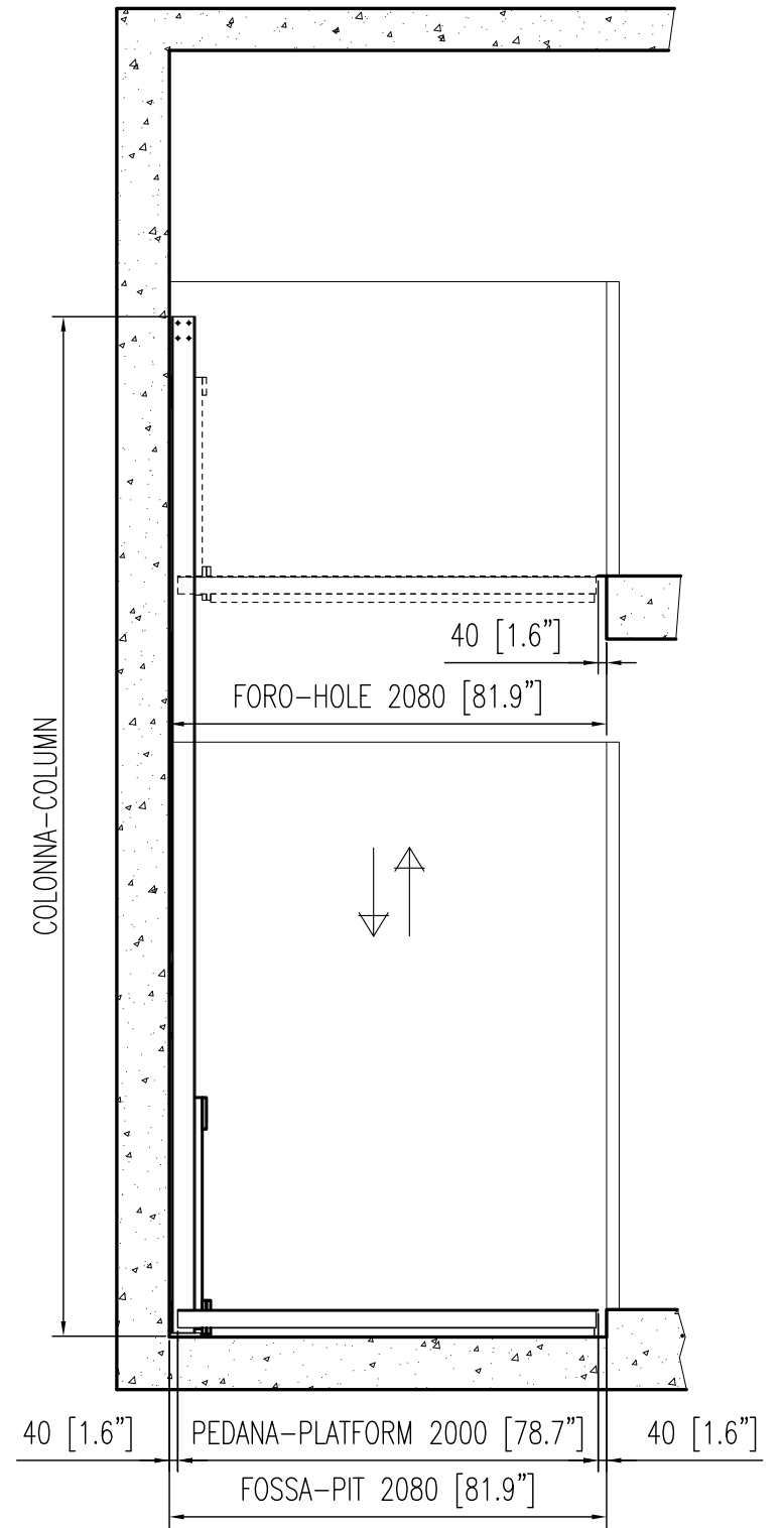
VISTA LATERALE SIDE VIEW
